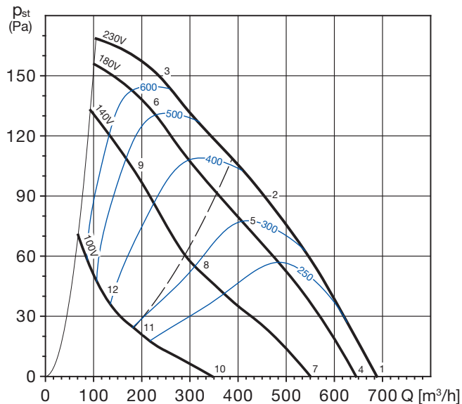
CRVB/4-250 N
