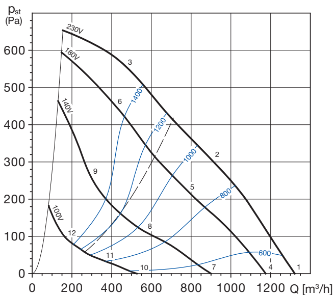
CRVB/2-250 N
