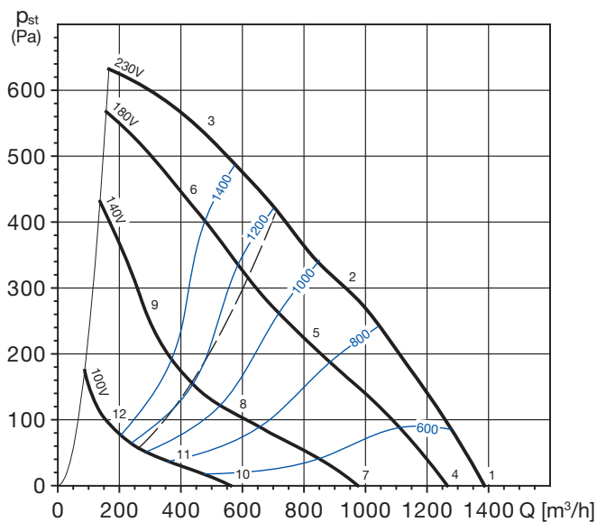
CRHB/2-250 N
