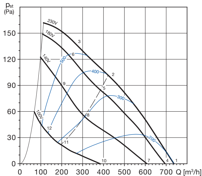
CRHB/4-250 N
